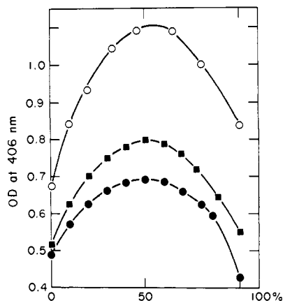
Figure 6. Plots of A_{406} vs. percent reduction of 3,10-dimethyl-8-cyanoisalloxazine ( 5 \times 10^{-5} M); C_2H_5NO_2 ( 2 \times 10^{-2} M) as reductant at pH 10.15 (○); C_6H_5SH ( 1 \times 10^{-3} M) as reductant at pH 9.90 (●) and at pH 10.15 (■).
