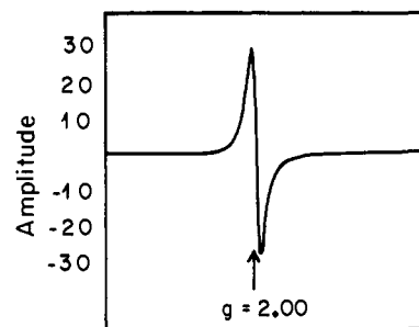
Figure 8. The EPR signal obtained at -35 °C from a half-reduced (52.7%) and frozen ( -35 °C) solution (pH 9.7, 0.10 M carbonate buffer) of 8-cyano-3,10-dimethylisalloxazine at 5.86 \times 10^{-5} M.
