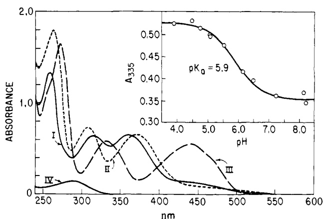
Figure 4. Curves I and II represent the spectra of reduced 8-cyano-10-methyl-3-sulfopropylisalloxazine ( 5.49 \times 10^{-5} M) at pH values of 4.49 and 8.15. Curve III is the spectrum of the oxidized isalloxazine. Curve IV represents the differential spectra obtained by subtracting the absorbance vs. nanometer plot of the product obtained upon reduction of the isalloxazine and reoxidation with \text{O}_2 , all at pH 8.15. This differential absorbance increases upon cyclic reduction and oxidation and represents decomposition products. Cyclic reduction and oxidation are quantitative at pH 7 and below. The inset represents the pH dependence of the absorbance of reduced isalloxazine. The points are experimental and the line represents a theoretical titration curve for a single proton ionization.
