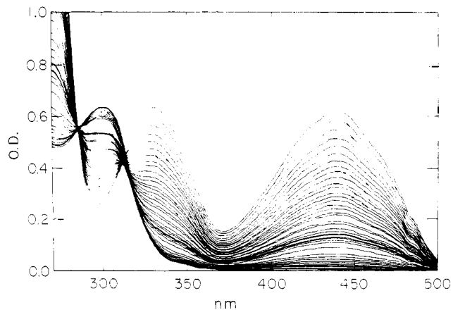
Figure 2. Repetitive spectral scan of the time course for the alkaline hydrolysis of 8-cyano-3,10-dimethylisoalloxazine ( 6.25 \times 10^{-5} M , pH 9.15, with 0.5 M carbonate buffer, 30 °C, solvent H_2O ).
