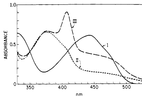
Figure 5. Plots of the absorbance spectra of oxidized (I), reduced (II), and half-reduced (III) 8-cyano-3,10-dimethylisalloxazine at a concentration of 5.8 \times 10^{-5} M and at pH 10.37. The typical anion radical absorbance at OD 406 (optical density) may be seen in plot III.
