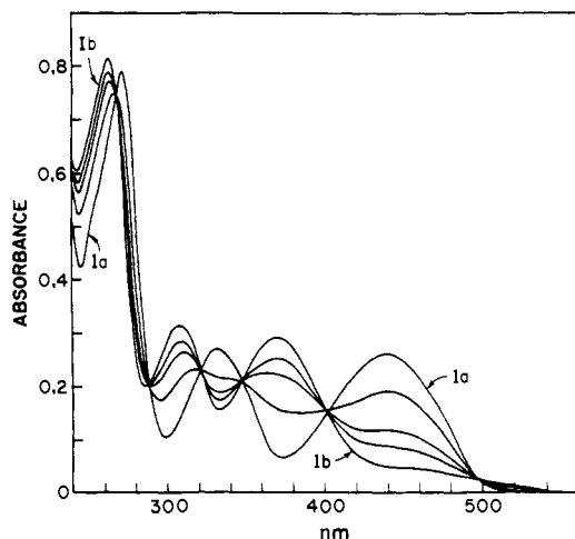
Figure 3. Repetitive spectral scans taken in the course of the reduction of 8-cyano-3,10-dimethylisalloxazine ( 2.52 \times 10^{-5} M) employing dithiothreitol as the reducing agent (pH 7.4, 0.1 M Tes buffer, \text{H}_2\text{O} , 30^\circ\text{C} ). Curves Ia and Ib represent the spectra of oxidized and reduced isalloxazine, respectively.
