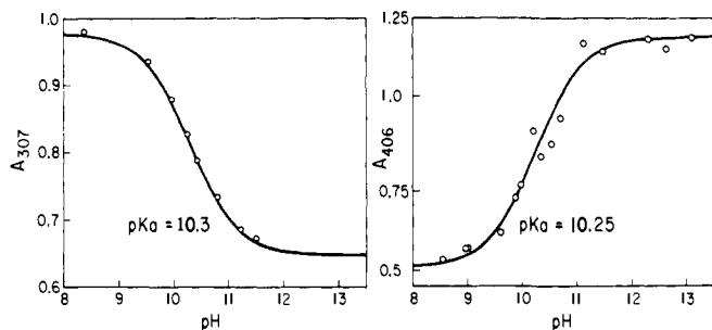
Figure 9. Plots of the absorbances at two wavelengths of half-reduced 8-cyano-3,10-dimethylisalloxazine vs. the adjusted pH (concentrations of XIa total are 2.5 \times 10^{-5} M for the measurements at A_{307} and 5 \times 10^{-5} M for those at A_{406} ).
