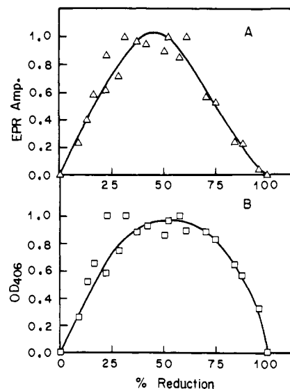
Figure 7. (A) Amplitude of the EPR signal obtained by freezing solutions (pH 9.7 carbonate buffer) at -35 °C vs. percent photocatalytic (with EDTA) reduction of 3,10-dimethyl-8-cyanoisalloxazine. (B) Absorbance of the same solutions at 406 nm plotted vs. percent reduction.
